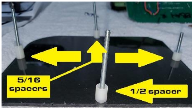
TACH - (1) THIS IS THE FIRST LAYER OF SPSCERS FOR TACH
